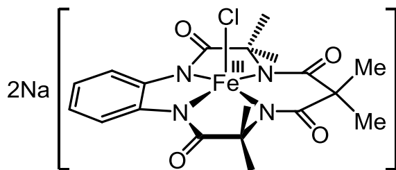
Figure 1. Molecular structure of the \text{Fe}(\text{TAML}^\text{®}) compound \text{FeB}^*
