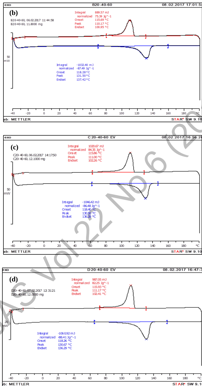
Figure 4. DSC curves of STF/NR/HDPE at different sizes of fibre (a) 1 mm, (b) 500 \mu m, (c) 250 \mu m and (d) 125 \mu m
