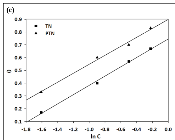
Figure 6. Adsorption mechanism of (a) Langmuir, (b) Freundlich and (c) Temkin isotherm for mild steel in 1 M HCl medium containing TN and PTN corrosion inhibitor
