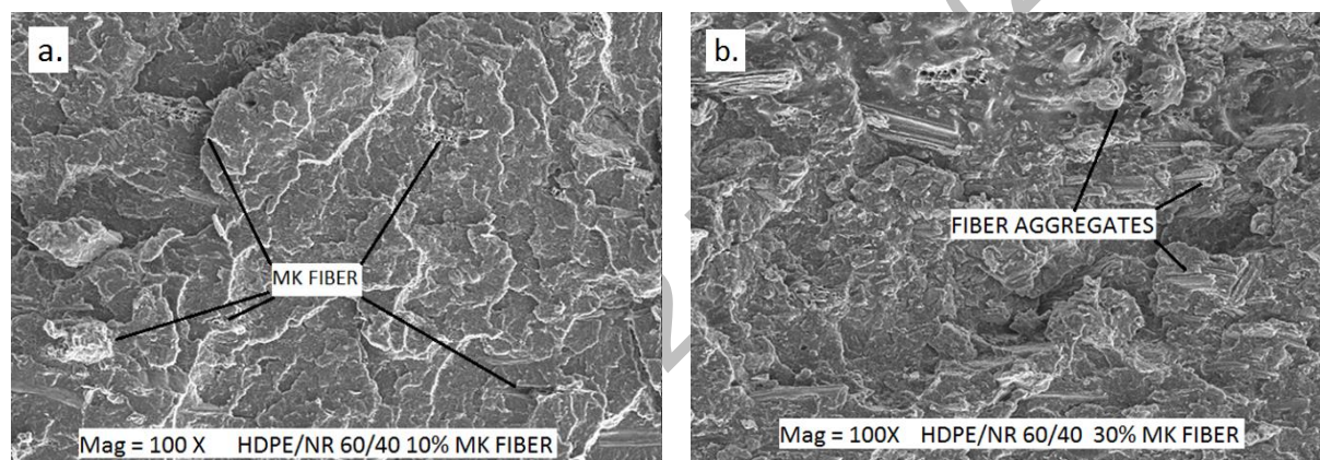
Figure 6. FESEM micrograph images of impact fracture surface on MK composites a) 40% rubber content and 10% MK fibre at 100 \times magnification, b) 40% rubber content and 30% MK fibre at 100 \times magnification
