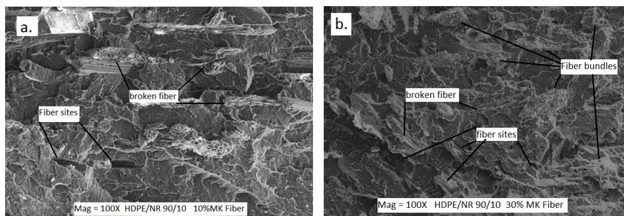
Figure 5. FESEM micrograph images of impact fracture surface on MK composites a) 10% rubber content and 10% MK fibre at 100 \times magnification, b) 10% rubber content and 30% MK fibre at 100 \times magnification
