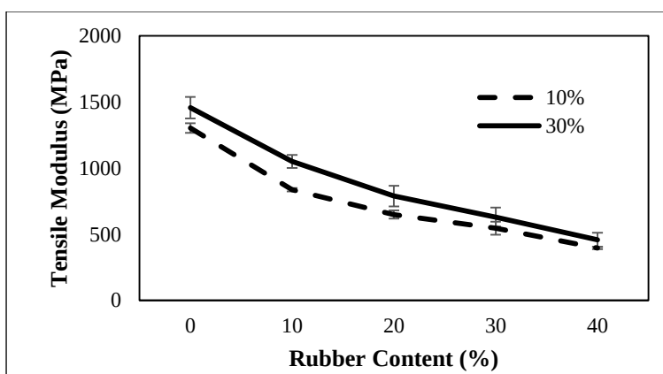
Figure 2. Tensile modulus of MK composites at 10% MK fibre and 30% MK fibre
