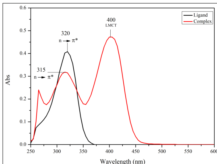
Figure 3. UV-Vis absorption spectra for compound HAcETSc and Sn(HAcETSc)PhenCl 2
