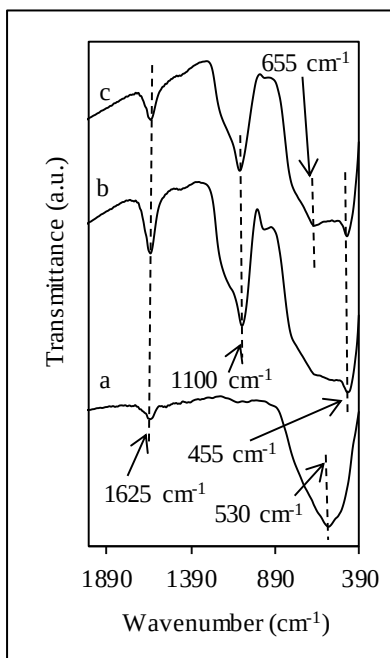
Figure 3. FTIR spectra in region 2000–390 \text{cm}^{-1} of (a) TiO 2 (b) MTN and (c) Ag-MTN
