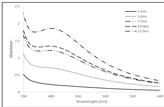
Figure 2. UV-Vis spectra of AgNPs synthesized at for various pomelo peel extract amount (Constant parameter: 1 mM \text{AgNO}_3 , 70 °C, 2 hours)
