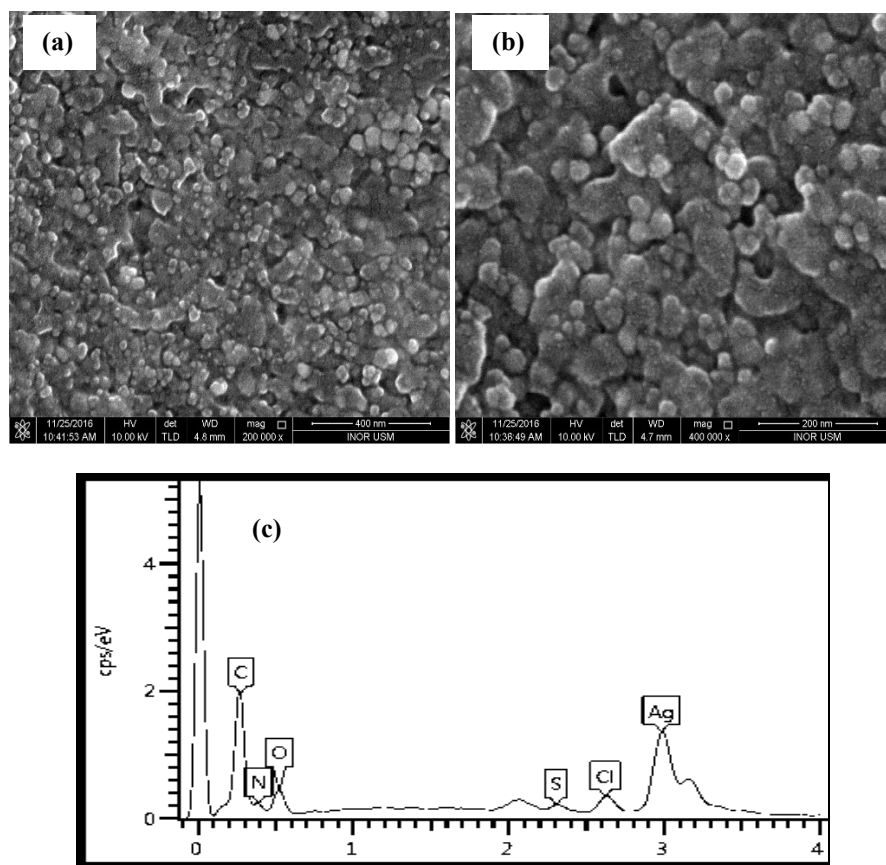
Figure 5. FESEM image of synthesized AgNPs at various resolutions (a) 200,000x, (b) 400,000x and (c) EDX profile showing the chemical composition (Condition of synthesized AgNPs: 2 mM \text{AgNO}_3 , 12.5 ml pomelo peel extract, 5 hours)
