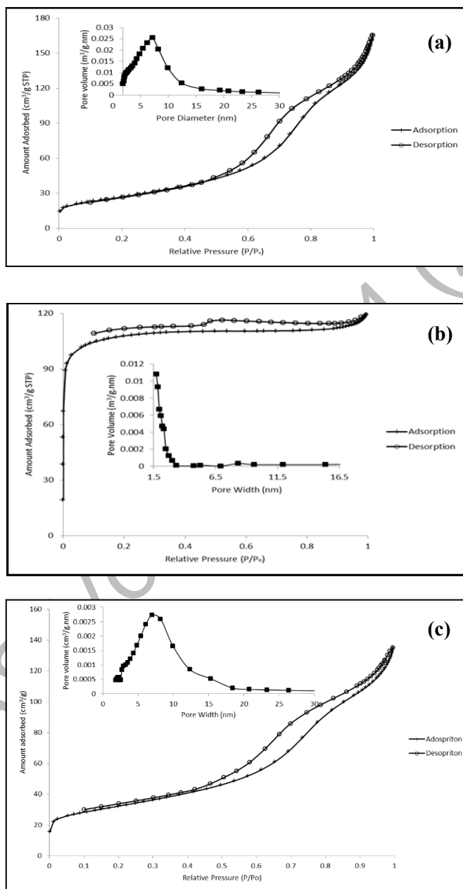
Figure 2. \text{N}_2 isotherm and pore distribution (inner graph) for (a) \text{TiO}_2 , (b) AC and (c) \text{TiO}_2/10\text{AC}
