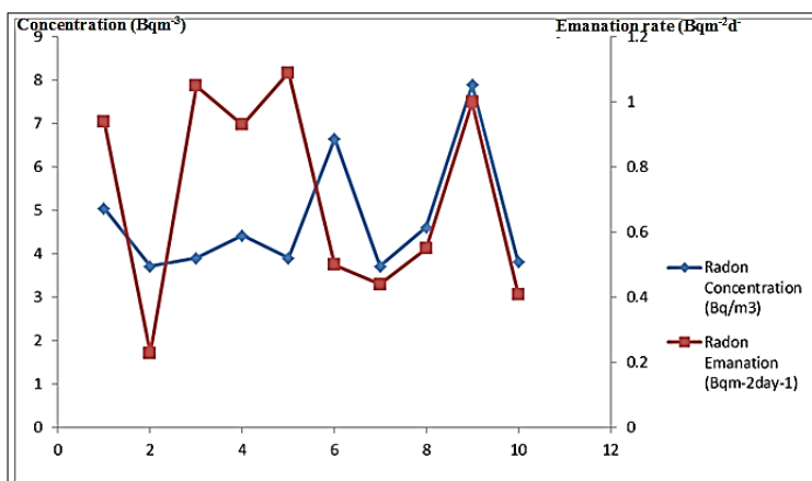
Figure 7. The relation between concentrations and emanation rates of Radon-222 according to sampling locations inside Gua Penyu cave
