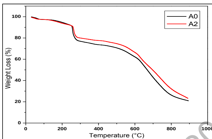
Figure 4. Thermal stability of synthesized ZIF-L samples with weight loss profile at different temperature and TEA/ total mole ratio: A0 (0) and A2 (0.0003)
