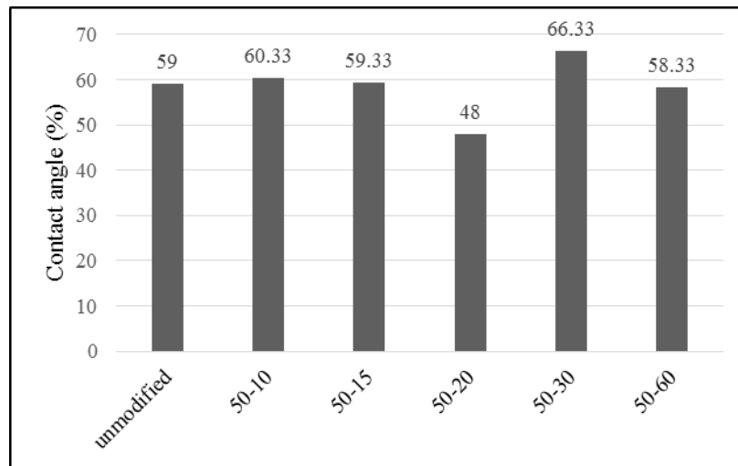
Figure 2. Hydrophilicity of the unmodified and modified membranes
