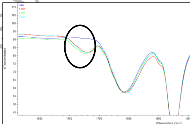
Figure 1. ATR-FTIR for modified and unmodified membranes at grafting time (1, 3 and 5 minutes)
