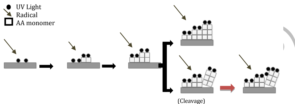
Figure 5. Proposed process on PES membrane surface. Modified from Taniguchi et al. [27].
