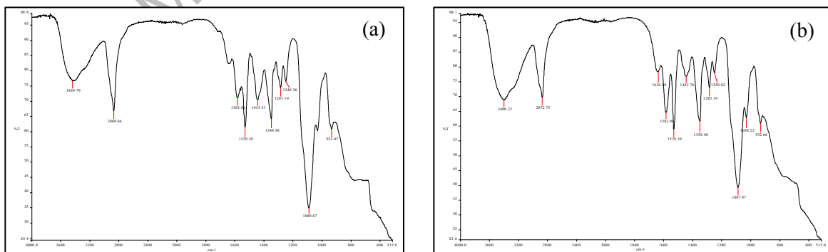
Figure 2. (a) FTIR pattern of \text{TiO}_2 -GAA powder, (b) FTIR pattern of \text{TiO}_2 - \text{HNO}_3 powder
