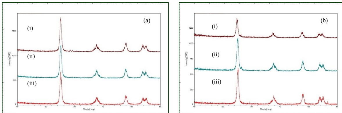
Figure 3. (a) XRD pattern of (i) 8 mmol GAA (ii) 9 mmol GAA (iii) 10 mmol GAA of \text{TiO}_2 powder, (b) XRD pattern of (i) 8 mmol \text{HNO}_3 (ii) 9 mmol \text{HNO}_3 (iii) 10 mmol \text{HNO}_3 of \text{TiO}_2 powder
