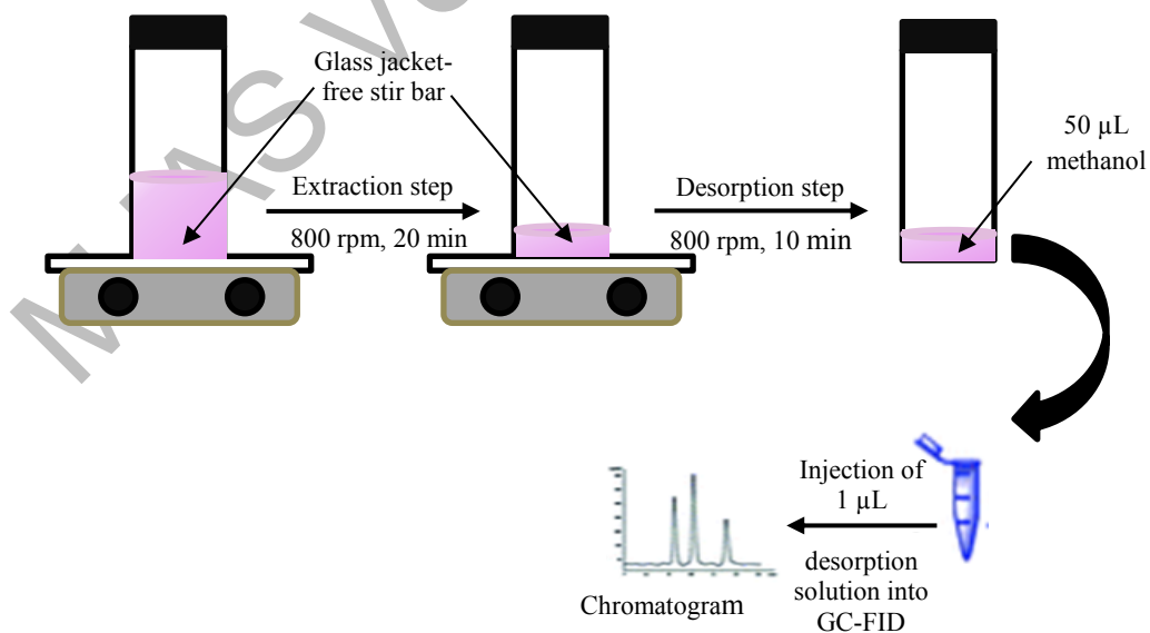
Figure 1. Schematic illustration of glass jacket-free SBSE process
