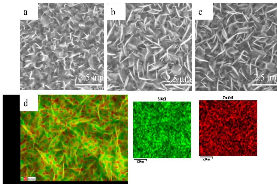
Figure 2. FESEM images of cobalt sulfide thin film deposited at (a) 5 (b) 10 (c) 15 minutes and d) is mapping picture to show the Co and S distribution (green color for sulfur and red color for cobalt)
