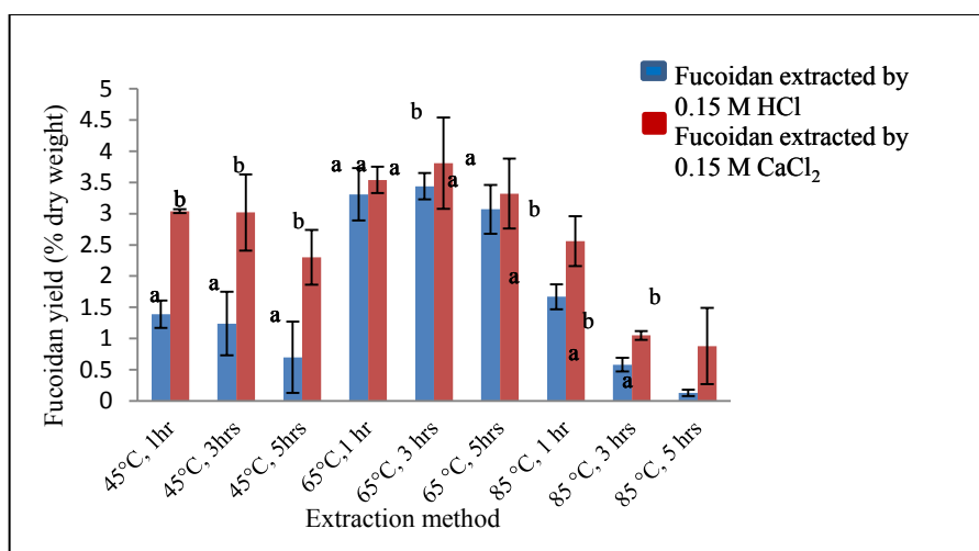
Figure 1. Graph of fucoidan yield (dry weight percentage) against the extraction method. a-b Different letters on fucoidan yield indicate a statistically significant difference ( p < 0.05 )
