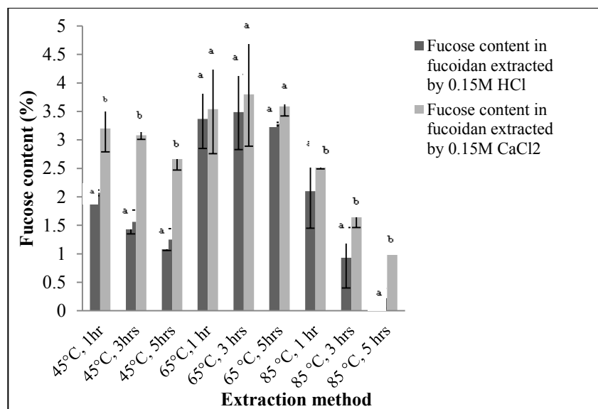
Figure 2. Graph of fucose content (%) against the extraction method. a-b Different letters on fucoidan yield indicate a statistically significant difference ( p < 0.05 )
