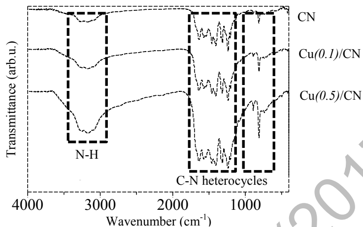
Figure 2. FTIR spectra of CN and Cu(x)/CN composites
