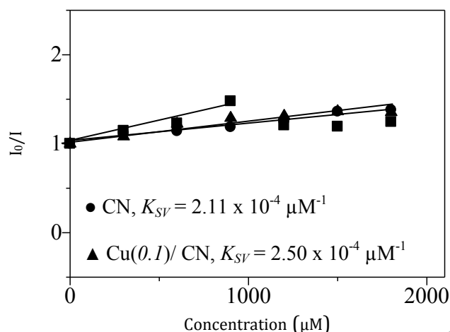
Figure 9. Stern-Volmer plots between the relative emission intensity of CN and Cu(x)/CN and the concentration of \text{NO}_3^- , monitored at excitation wavelength of C=N sites (277 nm)
