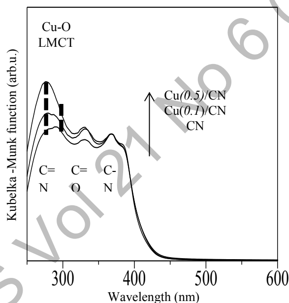
Figure 4. DR UV-Vis spectra of CN and Cu(x)/CN composites
