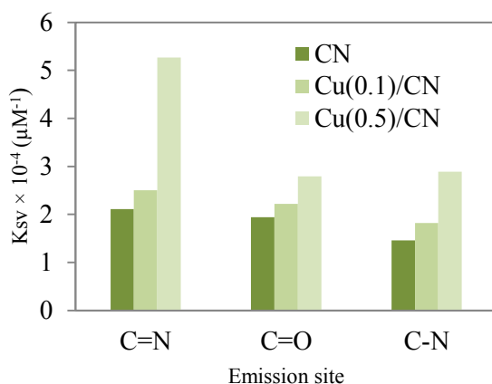
Figure 10. The K_{SV} values for CN and Cu(x)/CN for all the emission sites
