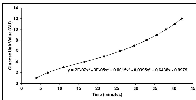
Figure 7. 5 th order calibration curve formed from 2-AA-Dextran profile for glucose unit (GU) value determination based on HPLC retention times
