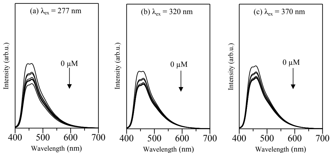
Figure 7. Emission spectra of Cu (0.1)/CN in the absence and presence of NO_3^- with various concentrations, monitored at excitation wavelength of (a) 277, (b) 320 and (c) 370 nm
