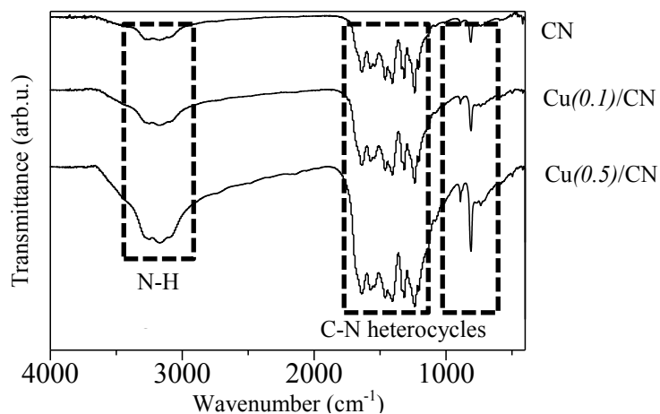
Figure 2. FTIR spectra of CN and Cu( x )/CN composites
