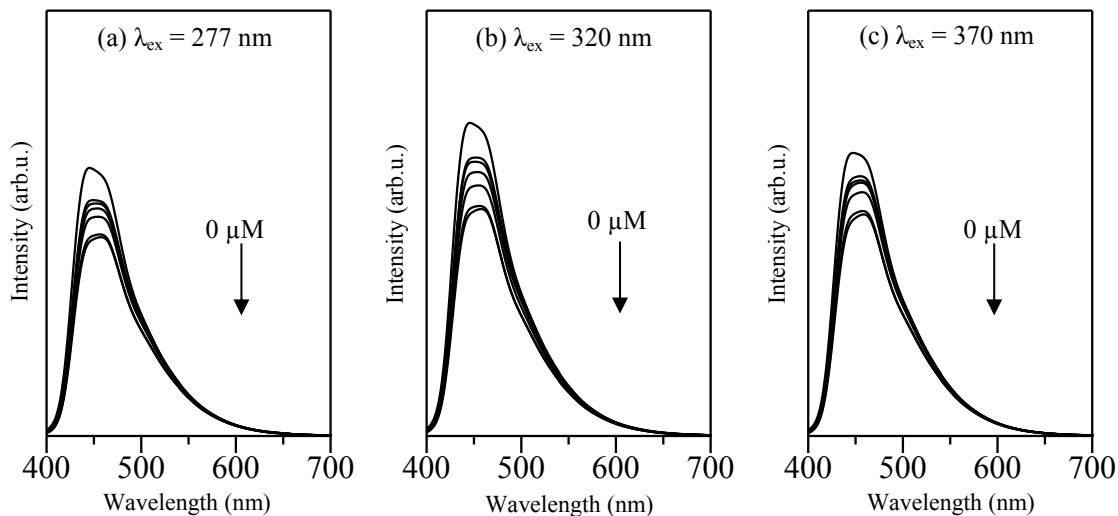
Figure 6. Emission spectra of CN in the absence and presence of NO_3^- with various concentrations, monitored at excitation wavelength of (a) 277, (b) 320 and (c) 370 nm
