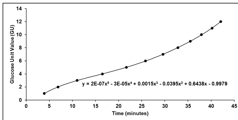
Figure 7. 5 th order calibration curve formed from 2-AA-Dextran profile for glucose unit (GU) value determination based on HPLC retention times
