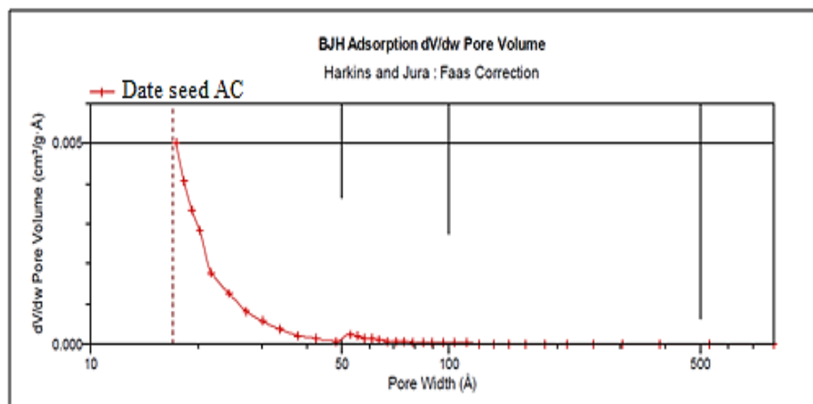
Figure 5. Pores size distribution plot of DAC
