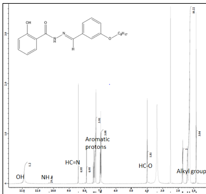
Figure 4. ^1\text{H} NMR spectrum of S8
