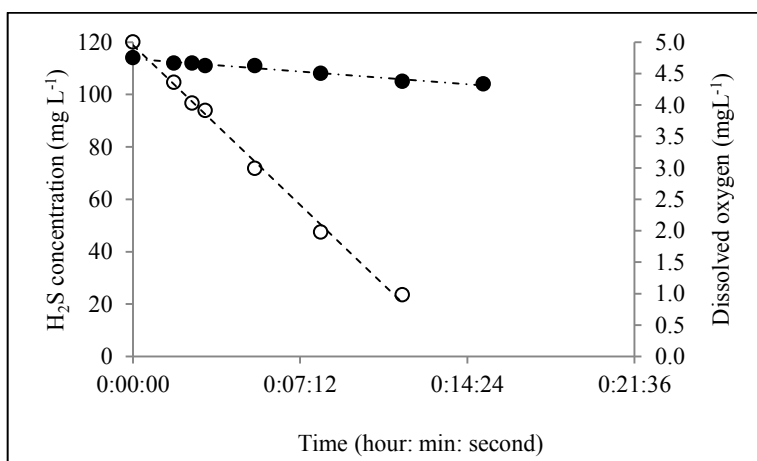
Figure 6. Typical hydrogen sulfide breakdown in seawater at low [\text{DO}/\text{H}_2\text{S}] concentration ratio [ \text{H}_2\text{S} initial concentration = 114 \text{ mg L}^{-1} ; DO initial concentration = 5 \text{ mg L}^{-1} ]. Open blank circle indicates dissolved oxygen while filled circle indicates concentration of hydrogen sulfide in seawater
