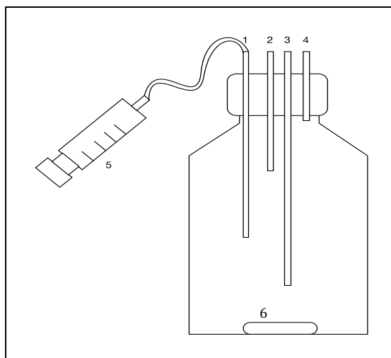
Figure 2. Experimental setup for investigating hydrogen sulfide solubility. 1. Piston inlet for sampling, 2. Gas inlet from Kipp's apparatus, 3. Sample outlet, 4. Excess gas exhaust, 5. Syringe, 6. Magnetic bar
