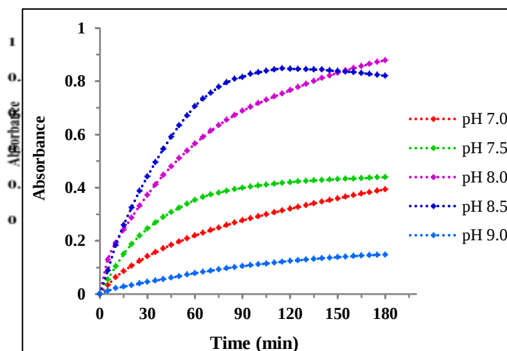
Figure 4. The response of sensor membrane at different pH with cadmium concentration of 2 ppm (n=3)
