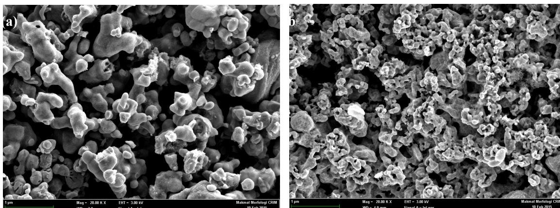
Figure 5. FESEM image of the surface of particle of (a) \text{Fe}_2\text{O}_3 and (b) \text{Rh-Fe}_2\text{O}_3 reduction at 650^\circ\text{C} in 10% CO atmosphere
