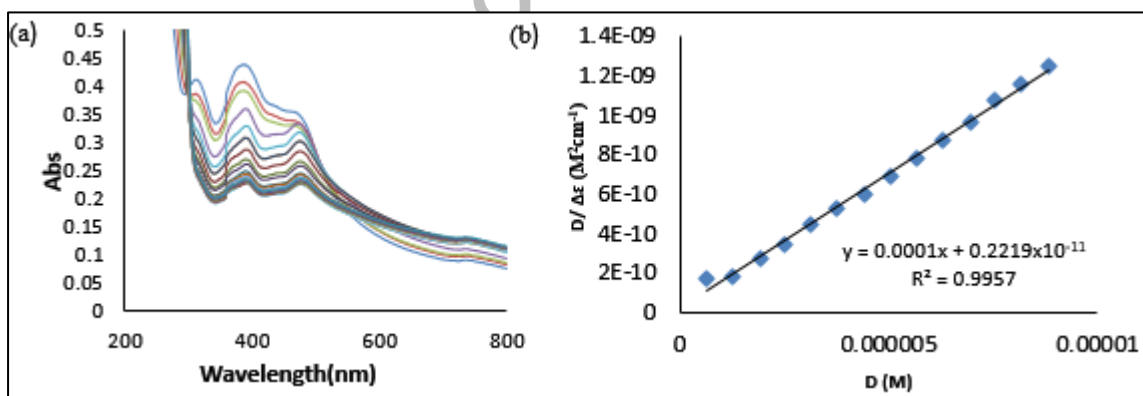
Figure 2. (a) Absorption spectral changes of complex [2] (30 μM) in Tris/KCl buffer (pH 7.4) in the absence and presence of increasing concentration of H-Telo (6.30 × 10 -3 mM – 1.3 × 10 -3 mM), (b) The reciprocal plot that fits the absorbance data to obtain the binding constant.
