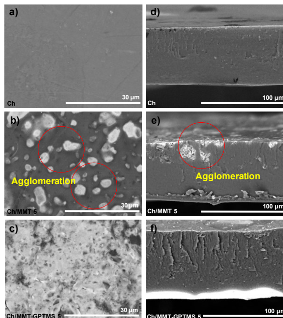
Figure 3. SEM images of (a) pristine Ch, (b) Ch/MMT, and (c) Ch/MMT-GPTMS membrane, (d), (e), and (f) showed the cross section of chitosan, Ch/MMT and Ch/MMT-GPTMS membrane, respectively
