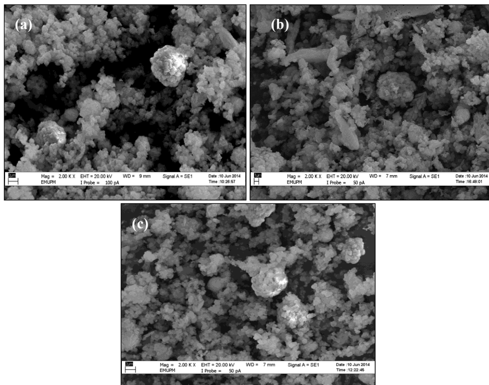
Figure 3. SEM micrograph of sample (a) 1:1, (b) 1:2, and (c) 2:1 at magnification 2000x
