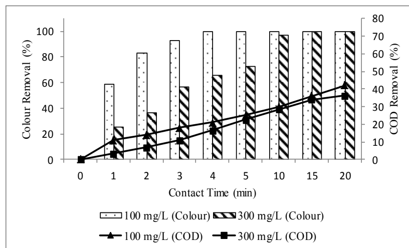
Figure 8. Effect of initial dye concentration on the colour and COD remov
