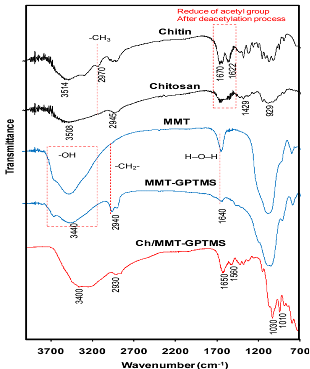
Figure 1. FTIR spectra of MMT, MMT-GPTMS, Chitin, Chitosan and Ch/MMT-GPTMS composite membrane
