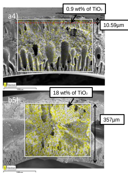
Figure 3. The EDX mapping of \text{TiO}_2 distribution in DLHF (a4) and SLHF (b5) membrane layer
