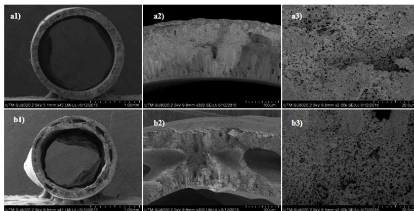
Figure 2. Cross-sectional and partial cross section FE-SEM images of the dual layer and single layer TiO 2 /PVDF hollow fiber membrane for (a) DLHF and (b) SLHF
