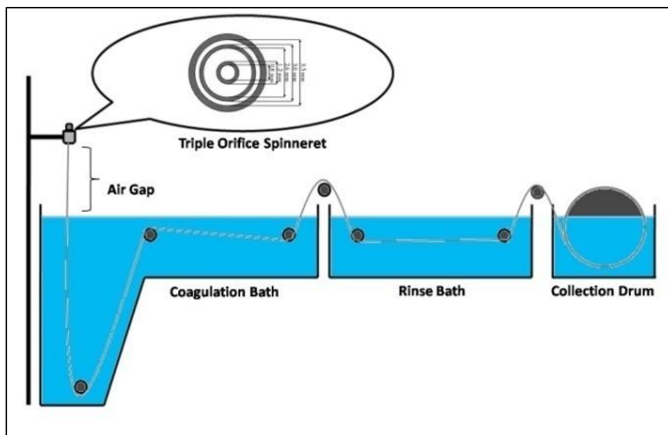
Figure 1. Dual layer hollow fiber spinning method
