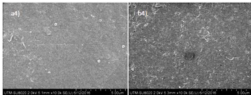
Figure 4. Surface FE-SEM images of the dual layer and single layer \text{TiO}_2 /PVDF hollow fiber membrane for (a) DLHF and (b) SLHF
