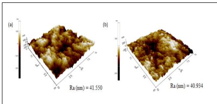
Figure 5. Surface roughness image of outer surface of (a) DLHF and (b) SHLF TiO 2 /PVDF hollow fiber membranes
