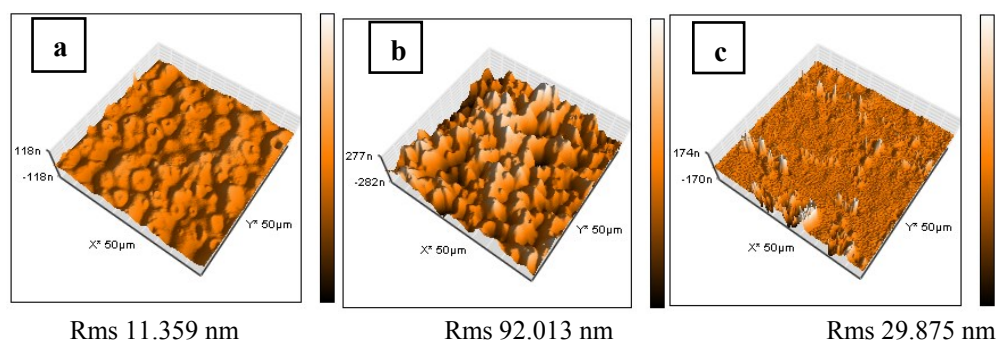
Figure 5. AFM micrographs of B1 (a), B2 (b), and A4(c) membranes after plasma treatment
