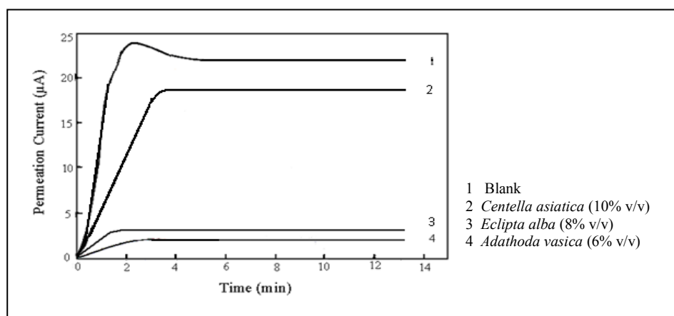
Figure 8. Hydrogen permeation current vs. time plots for mild steel in 1N HCl solution in the absence and presence of an optimum concentration of the plant extracts
