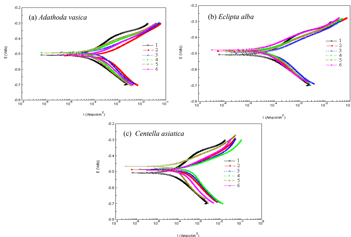
Figure 1. Potentiodynamic polarization curves for mild steel in 1N HCl solution in the absence and presence of various concentrations of the plant extracts (a) Adathoda vasica , (b) Eclipta alba and (c) Centella asiatica (Note legend information: 1 – blank, 2 – 2.0% v/v, 3 – 4.0% v/v, 4 – 6.0% v/v, 5 – 8.0% v/v and 6 – 10.0% v/v)
