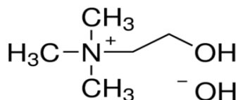
Figure 1. The ionization structure of choline hydroxide
