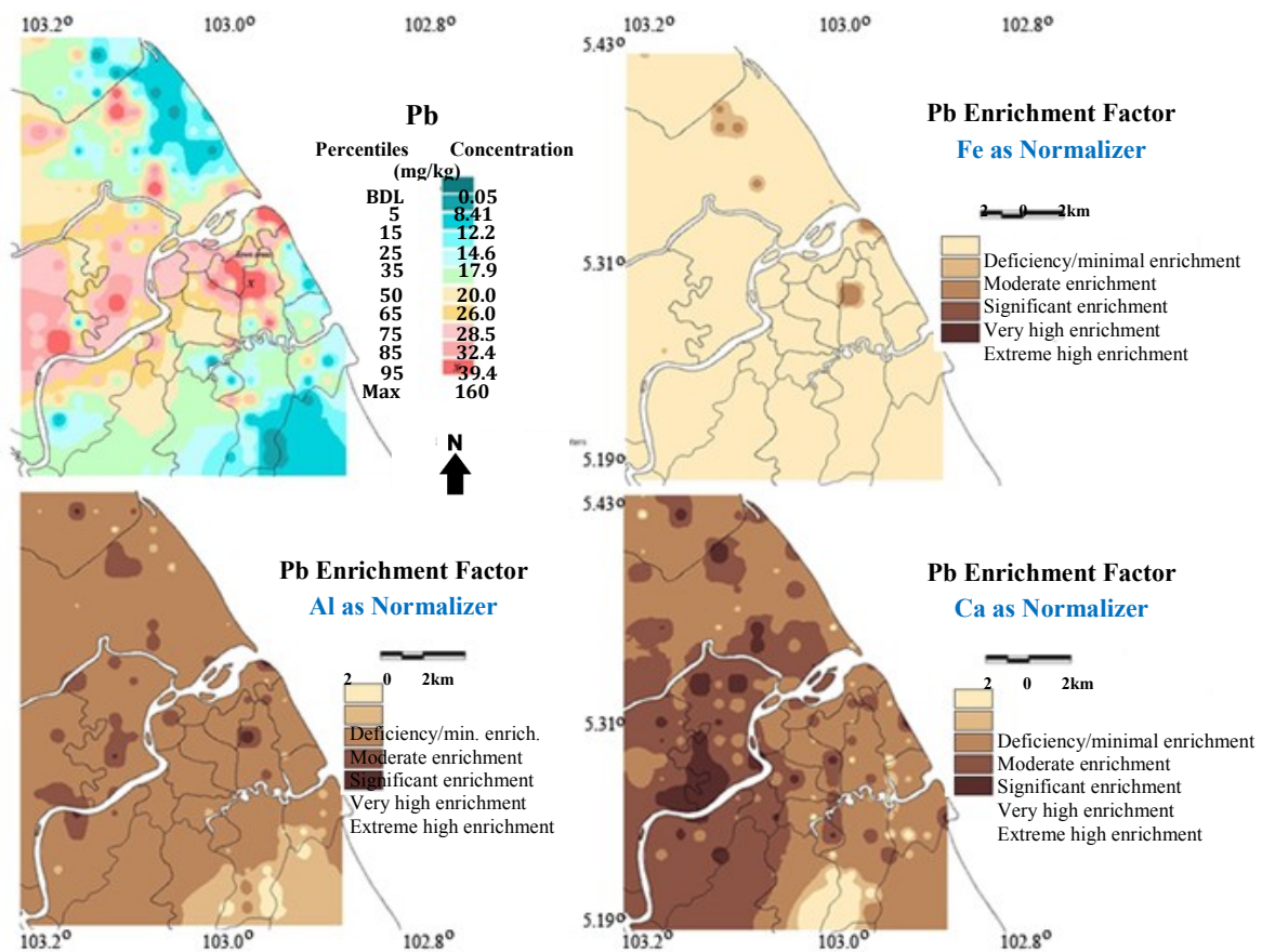
Figure 3. Comparison of the calculated EFs for Pb in Kuala Terengganu soils
