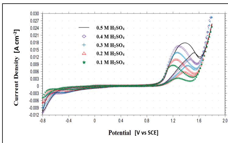
Figure 3. Cyclic voltammogram of stainless steel electrodes using different concentration of sulfuric acid in the absence of thiourea
