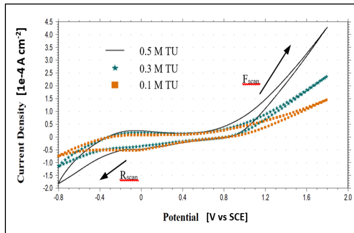
Figure 4. Cyclic voltammogram of stainless steel electrodes using different concentration of TU in the absence of sulfuric acid
