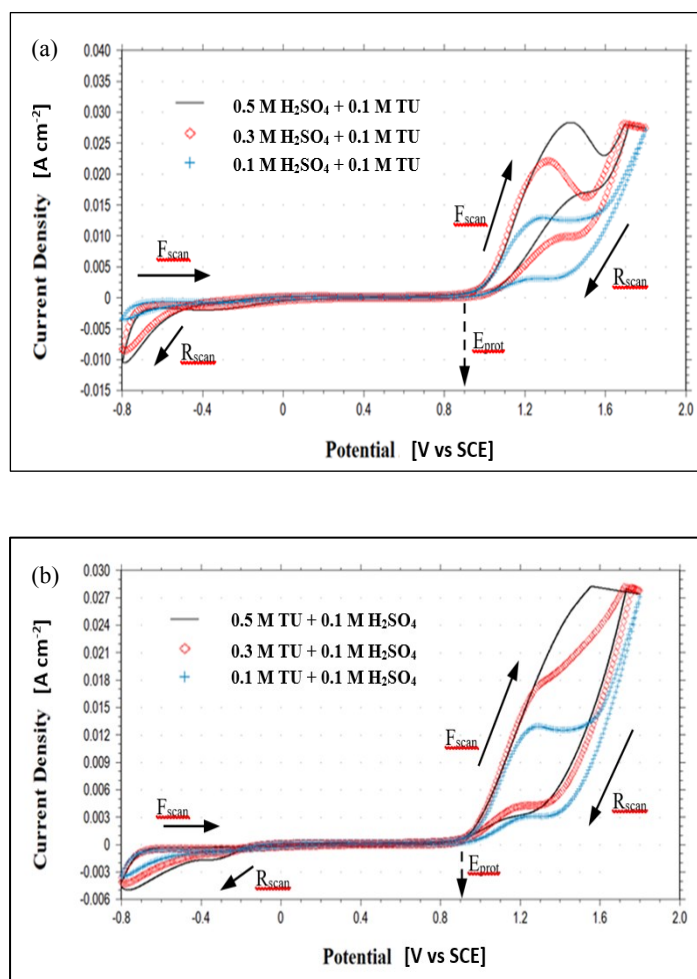
Figure 2. Cyclic voltammogram of stainless steel electrodes in the acidic thiourea solution for fixed (a) concentration of thiourea and (b) concentration of sulfuric acid
