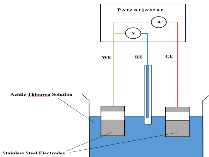
Figure 1. Experimental setup for 3-electrode system of CV study on corrosion of stainless steel electrode in acidic thiourea solution
