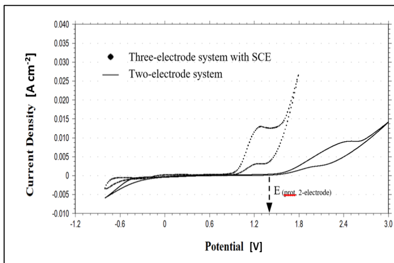
Figure 5. Cyclic voltammogram of stainless steel electrodes using (●) three-electrode system with saturated calomel electrode (SCE) as reference electrode, and (—) two-electrode system
