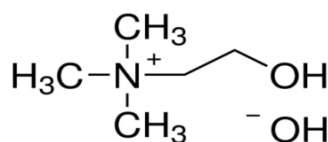
Figure 1. The ionization structure of choline hydroxide
