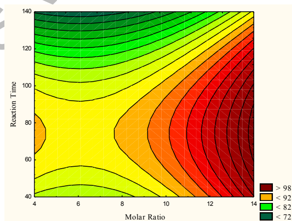
Figure 7. Contour plot of molar ratio ethanol: CPO and reaction time against percentage yield
