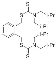
Figure 1. Structure of ionophore o-xylylene bis(N,N-diisobutyldithiocarbamate) (o-xc)
