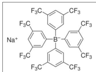
Figure 4. NaTFPB molecule with negatively charged B
