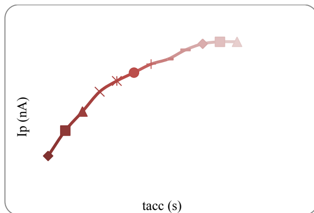
Figure 6. Effect of various t_{acc} on the I_p of second reduction peak of 2 mg/L RB5 dye in BRB solution at pH 2.5. Initial instrumental parameters were E_i = +150 mV, E_f = -650 mV, v = 5 mV/s, E_{acc} = 0 mV and pulse amplitude = 50 mV
