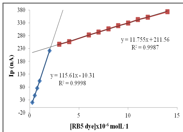
Figure 8. Two linear curves of RB5 dye in BRB solution at pH 2.5. (a) 2.5 \times 10^{-7} to 2.0 \times 10^{-6} \text{ mol L}^{-1} and (b) 3.0 \times 10^{-6} to 1.4 \times 10^{-5} \text{ mol L}^{-1}
