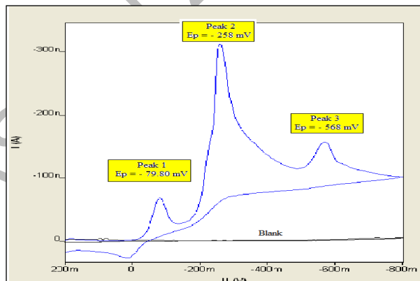
Figure 2. Cyclic voltammogram of 2 \times 10^{-4} \text{ molL}^{-1} RB5 dye in BRB solution at pH 4.0. Experimental condition: E_i = +200 \text{ mV} , E_{switch} = -800 \text{ mV} , E_f = +200 \text{ mV} and \nu = 25 \text{ mV/s}
