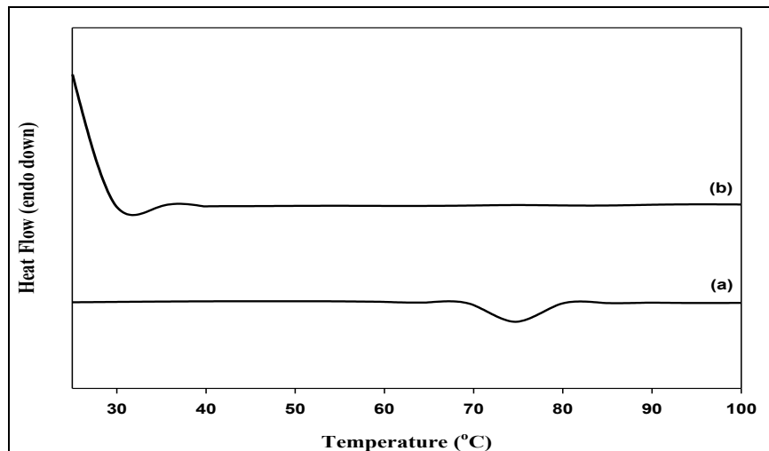
Figure 5. DSC thermogram of (a) native starch and (b) S-ETAC (DS = 0.11)
