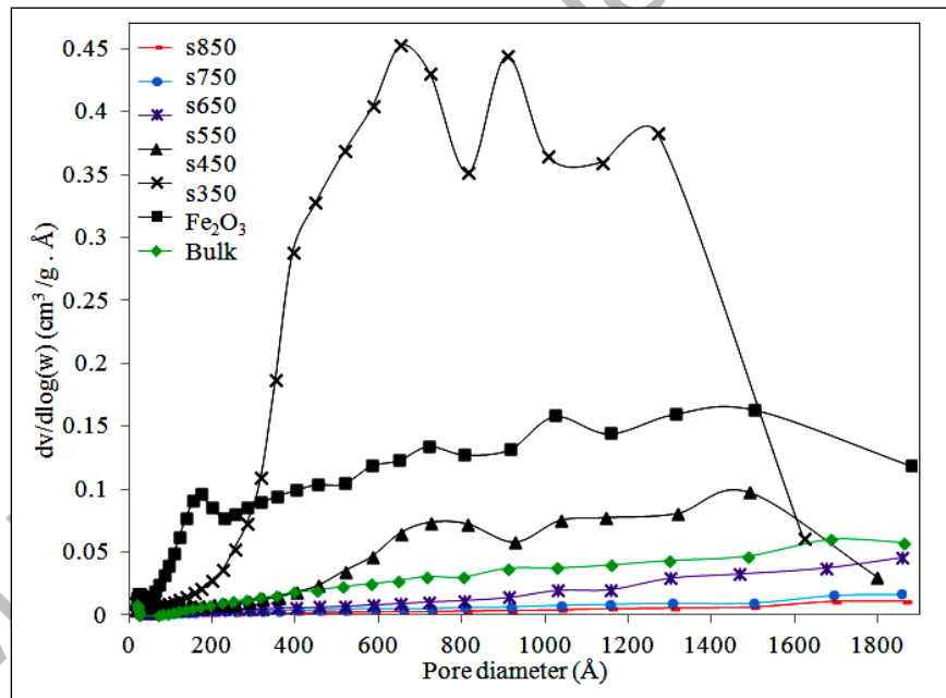
Figure 3. Pore size distribution of synthesized \alpha\text{-Fe}_2\text{O}_3 by BJH method
