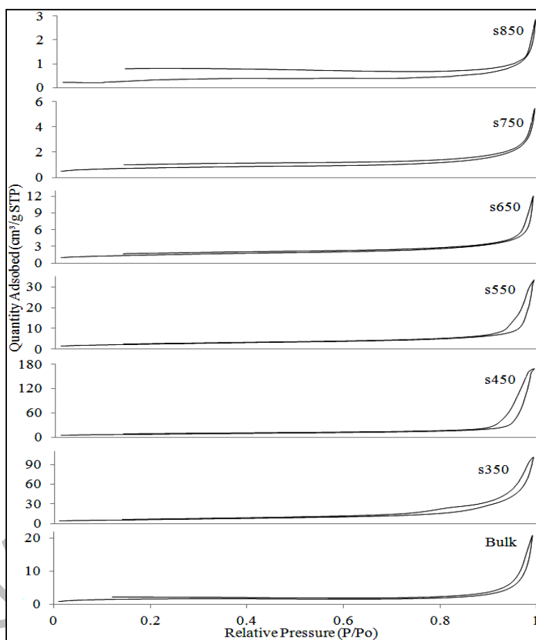
Figure 2. The effect of calcination temperature on \alpha\text{-Fe}_2\text{O}_3 towards \text{N}_2 adsorption-desorption isotherms
