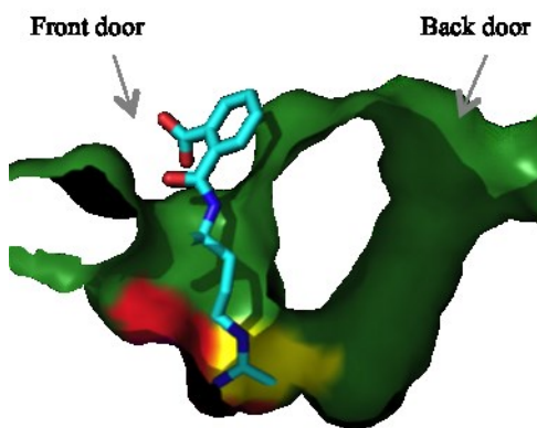
Figure 2. Two accessible doors of PAD4 catalytic pocket. Ligand such as o-F-amidine (rendered as blue stick) is bound at the front door. The main catalytic residue C645 is colored in yellow and H471 is colored in red.
