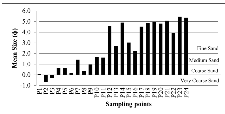
Figure 4. Variation of mean sediment size ( \phi ) in surficial sediments of Sungai Pinang, Penang
