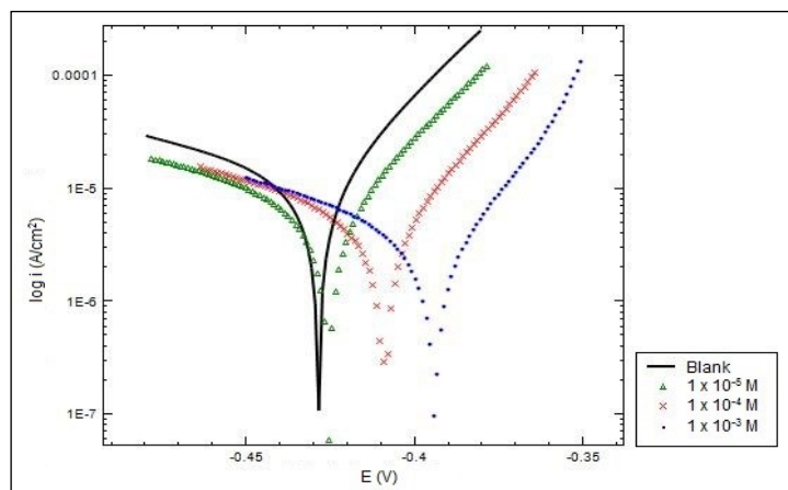
Figure 6. Polarization curves of various concentration of compound C in 1.0 M H 2 SO 4
