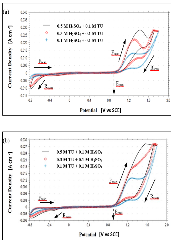
Figure 2. Cyclic voltammograms of stainless steel electrodes in the acidic thiourea solution for fixed (a) concentration of thiourea and (b) concentration of sulfuric acid
