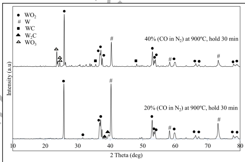
Figure 3. XRD profile for isothermal reduction of WO_2 by 20 and 40 % ( CO in N_2 ) up to 900^\circ C and hold for 30 min
