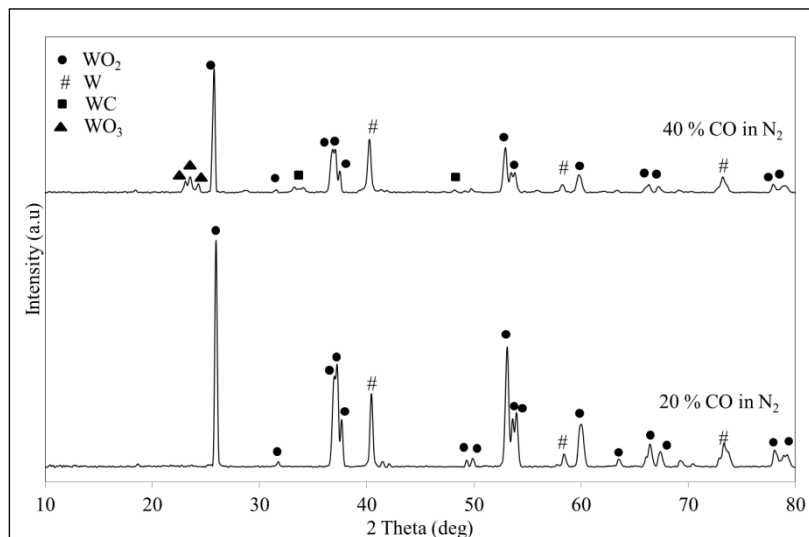
Figure 2. XRD profile obtained for non-isothermal reduction of WO_2 by 20% and 40% ( CO in N_2 ) up to 900^\circ C
