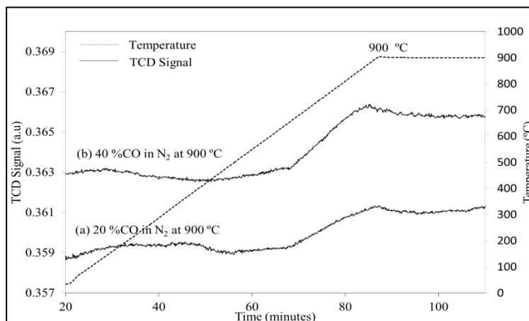
Figure 1. TPR profile obtained for non-isothermal and isothermal reduction of \text{WO}_2 by 20% and 40% (CO in \text{N}_2 ) up to 900^\circ\text{C} and hold for 30 minutes respectively
