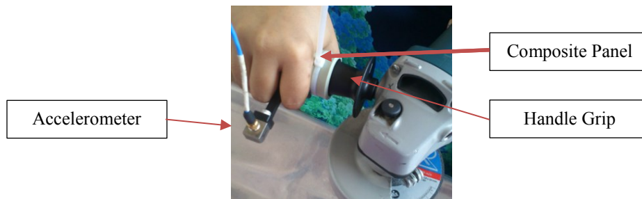
Figure 1. Hand grinder grip attached with composite panels and accelerometer
