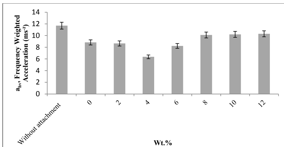
Figure 5. Sum average frequency weighted acceleration
