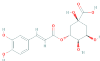
Figure 1. Chemical structure of chlorogenic acid (CGA)
