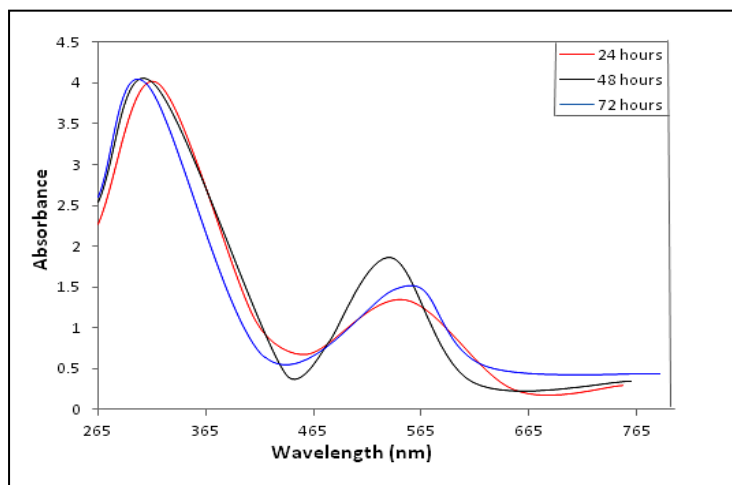
Figure 2. UV-Vis spectra of P(ANI- co-m -ABA) at 24, 48 and 72 hours, respectively
