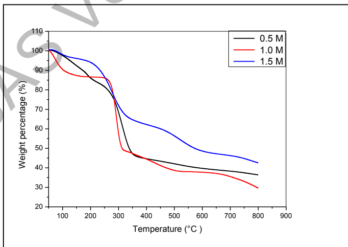
Figure 5. TGA thermograms of P(ANI-co-m-ABA)/PS composite nanofibers at different concentrations
