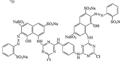
Figure 1. Chemical structures and physical properties of AB29, RO16 and RR120
