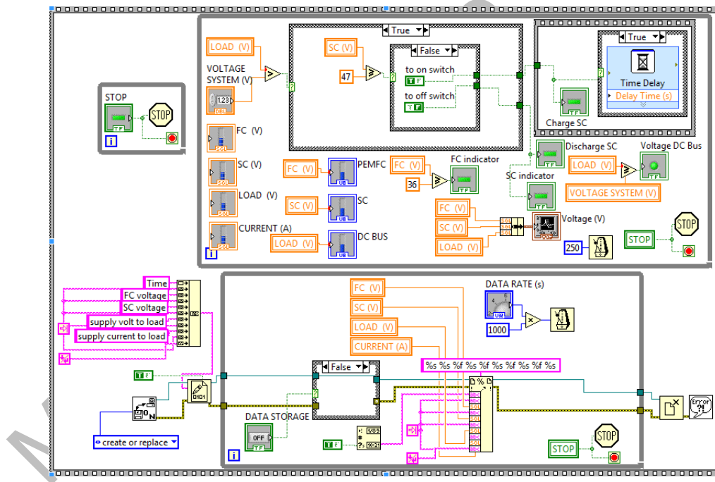
Figure 7. Block diagram of power management program
