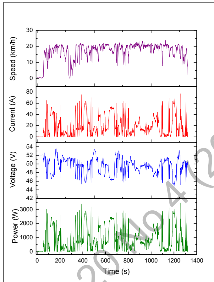
Figure 9. Measurement of speed, current, voltage and power response during on road testing using BT as power generator
